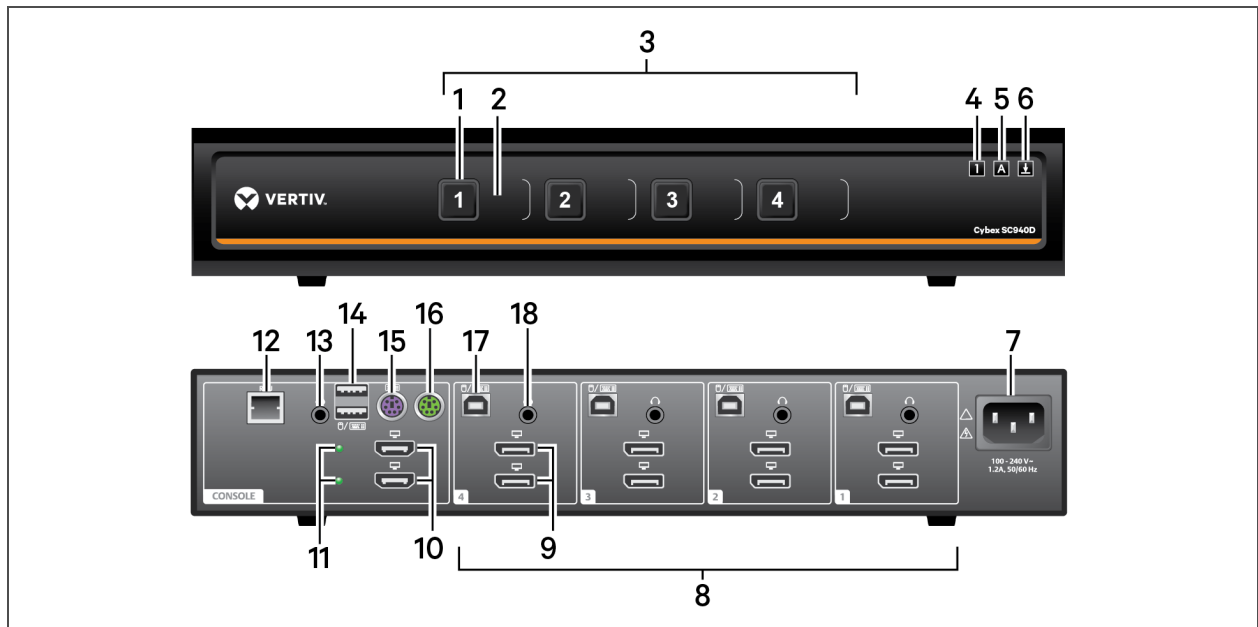
Figure 2.5 SC 940D KVM Switch
